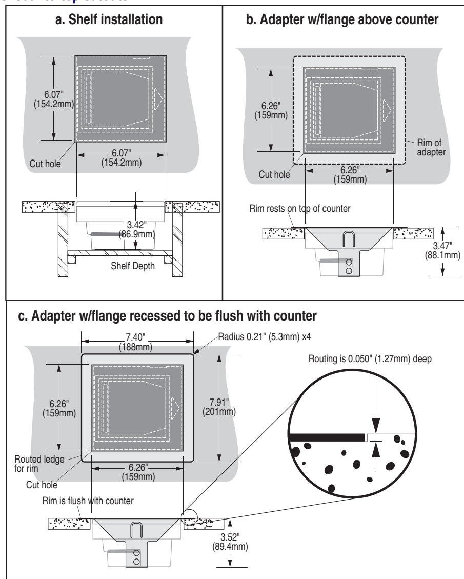
Figure 3. Countertop Cutouts
